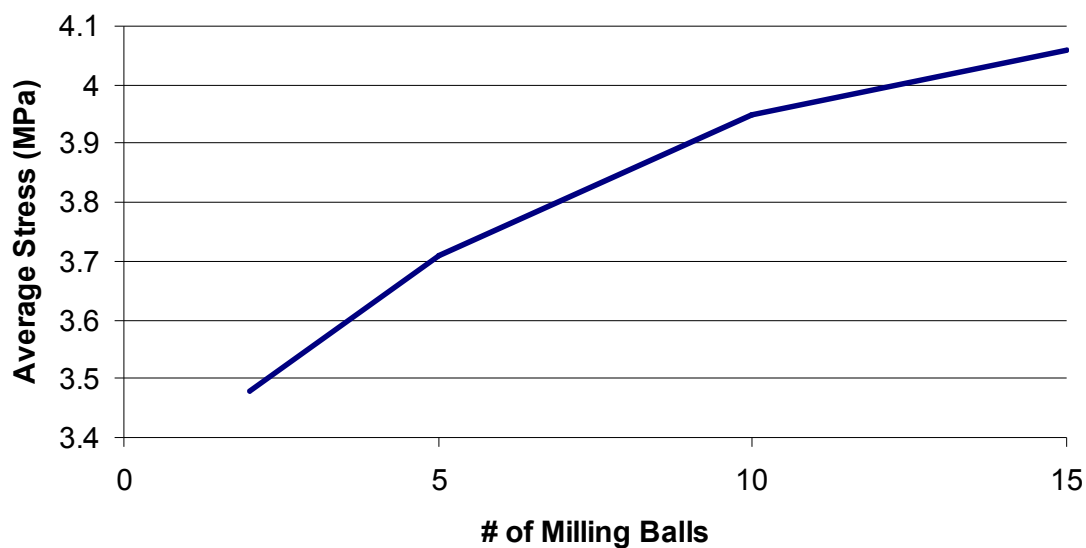
Figure 9: Average film impact stress as a function of the number of milling balls for low film on PT001.
