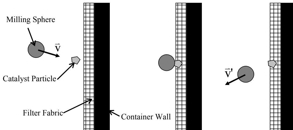
Figure 2: Schematic of catalyst impregnation via sphere-particle-fabric impact
