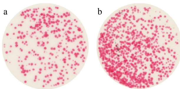
Figure 5: Impacts on pressure sensitive film on bare steel vial wall after 5 seconds of milling with a) 5 PMMA balls and b) 15 PMMA balls.
