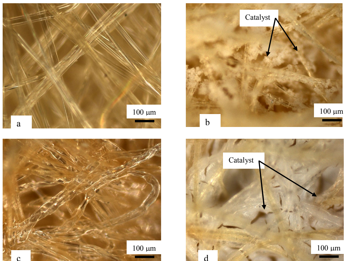
Figure 3: Darkfield images of a) pristine PT001, b) PT001 milled with 10-75 \mu\text{m} \text{Al}_2\text{O}_3 with water, c) pristine RY805, and d) RY805 milled with nanometer \text{Al}_2\text{O}_3 and 70% isopropyl alcohol. Note the agglomeration of nanometer \text{Al}_2\text{O}_3 into micrometer-sized clumps.
