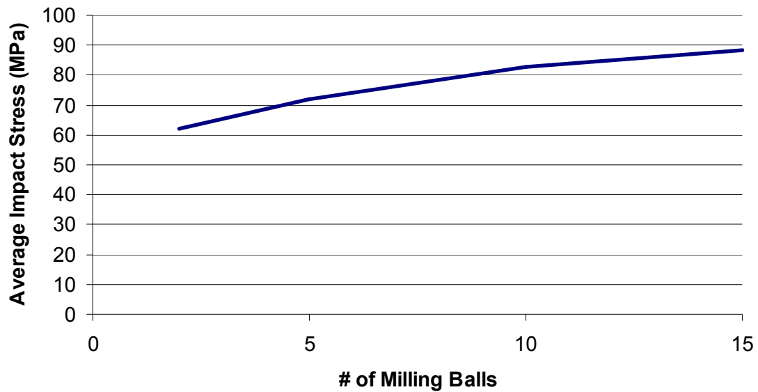
Figure 7: Average film impact stress as a function of the number of milling balls for high film on bare steel.
