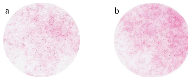
Figure 8: Impacts on pressure sensitive film on PT001 after 5 seconds of milling with a) 5 PMMA balls and b) 15 PMMA balls.
