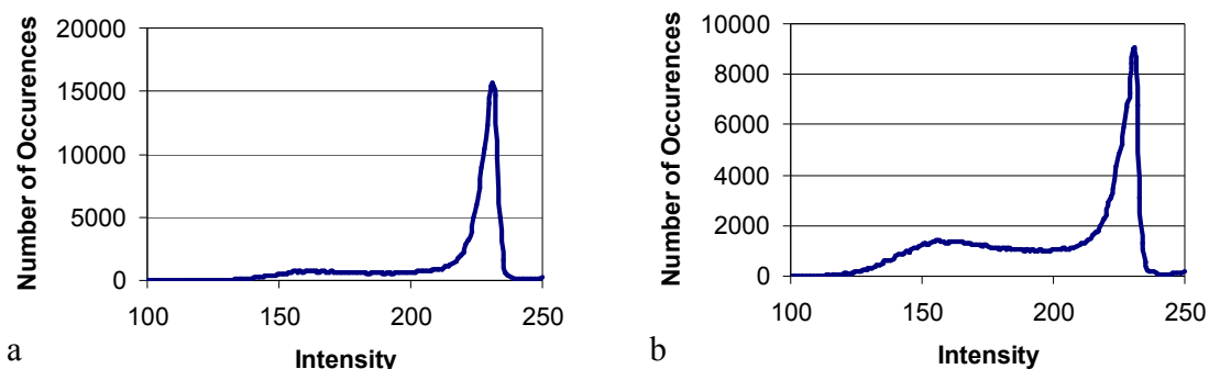
Figure 6: ImageJ analysis of pressure film results for bare steel with a) 5 PMMA balls and b) 15 PMMA balls.
